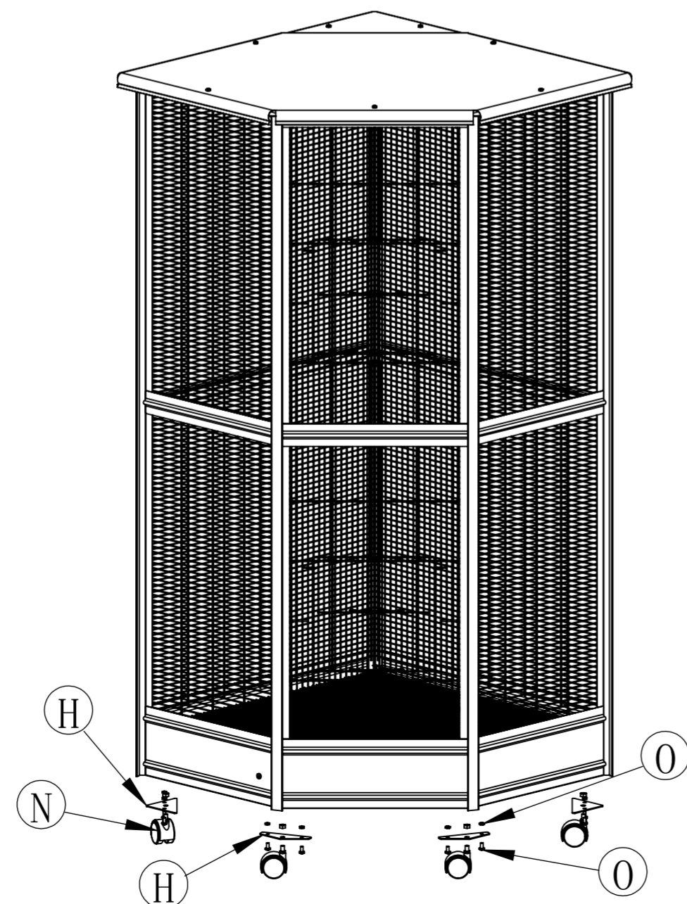
5、Screw the triangle plates H and wheels N to the cage bottom.
