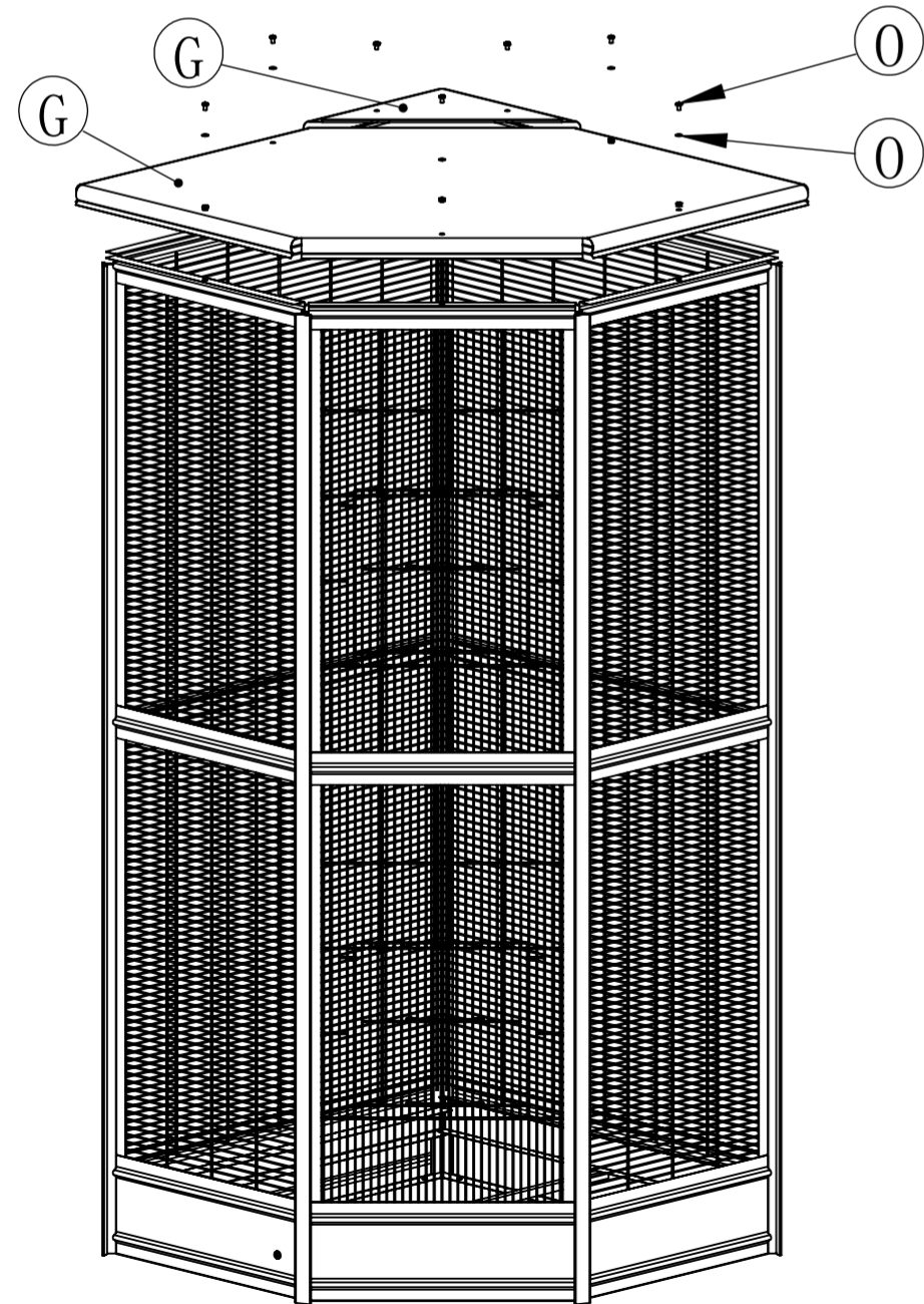
4、Screw roof G to the cage body with O.
