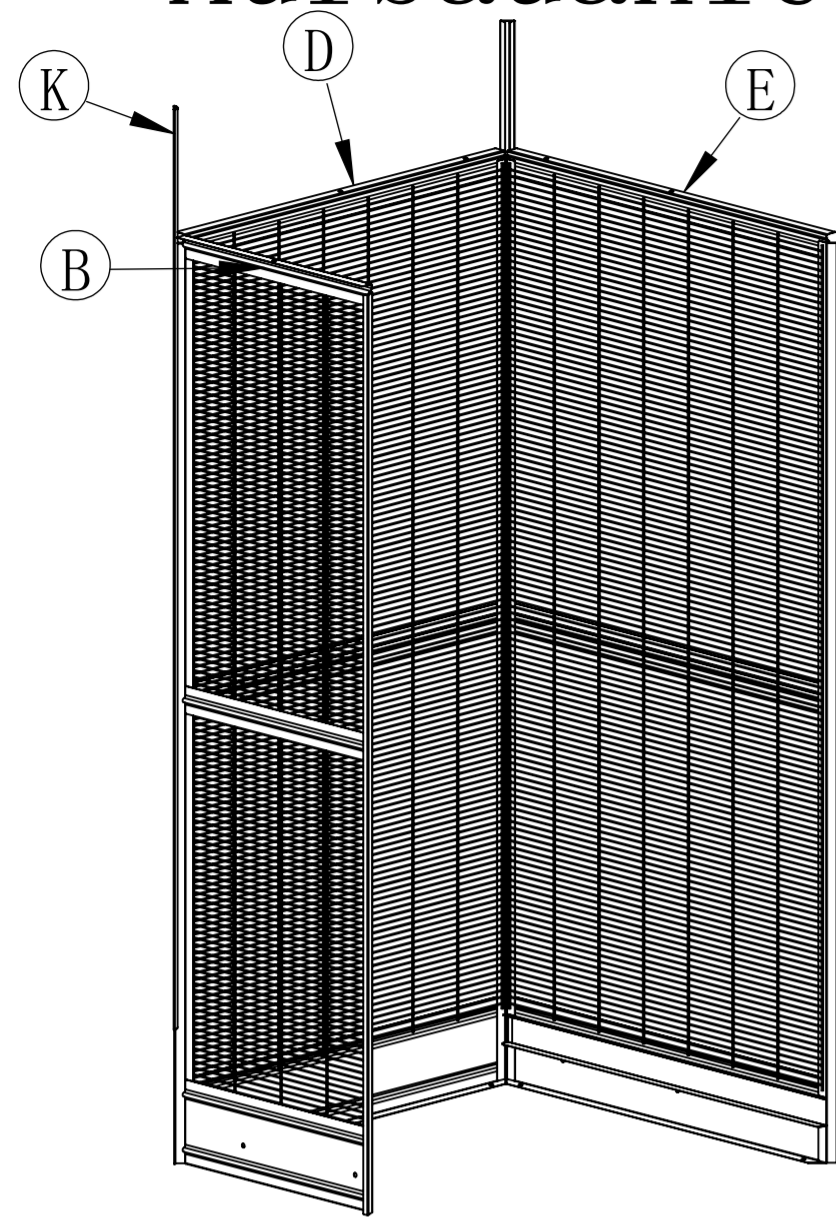
1、Attach part B, D and E with K(attaching clamp)
