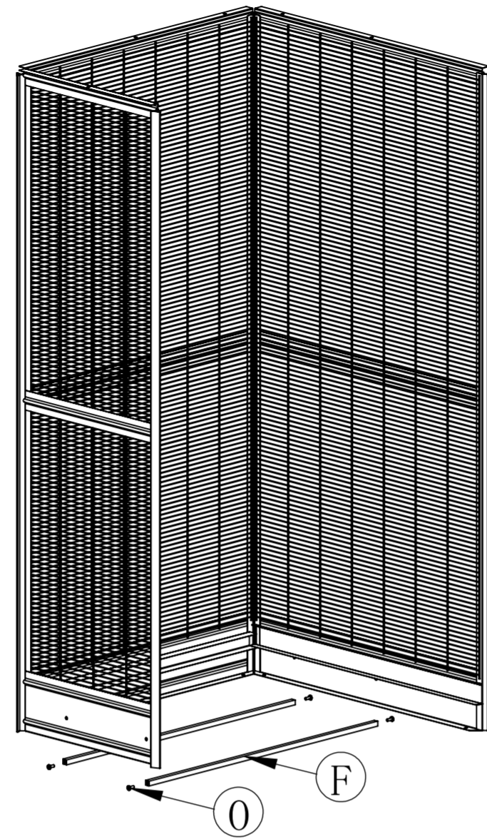
2、Attach left panel B and back right Panel E with frame bar F and screws O.
