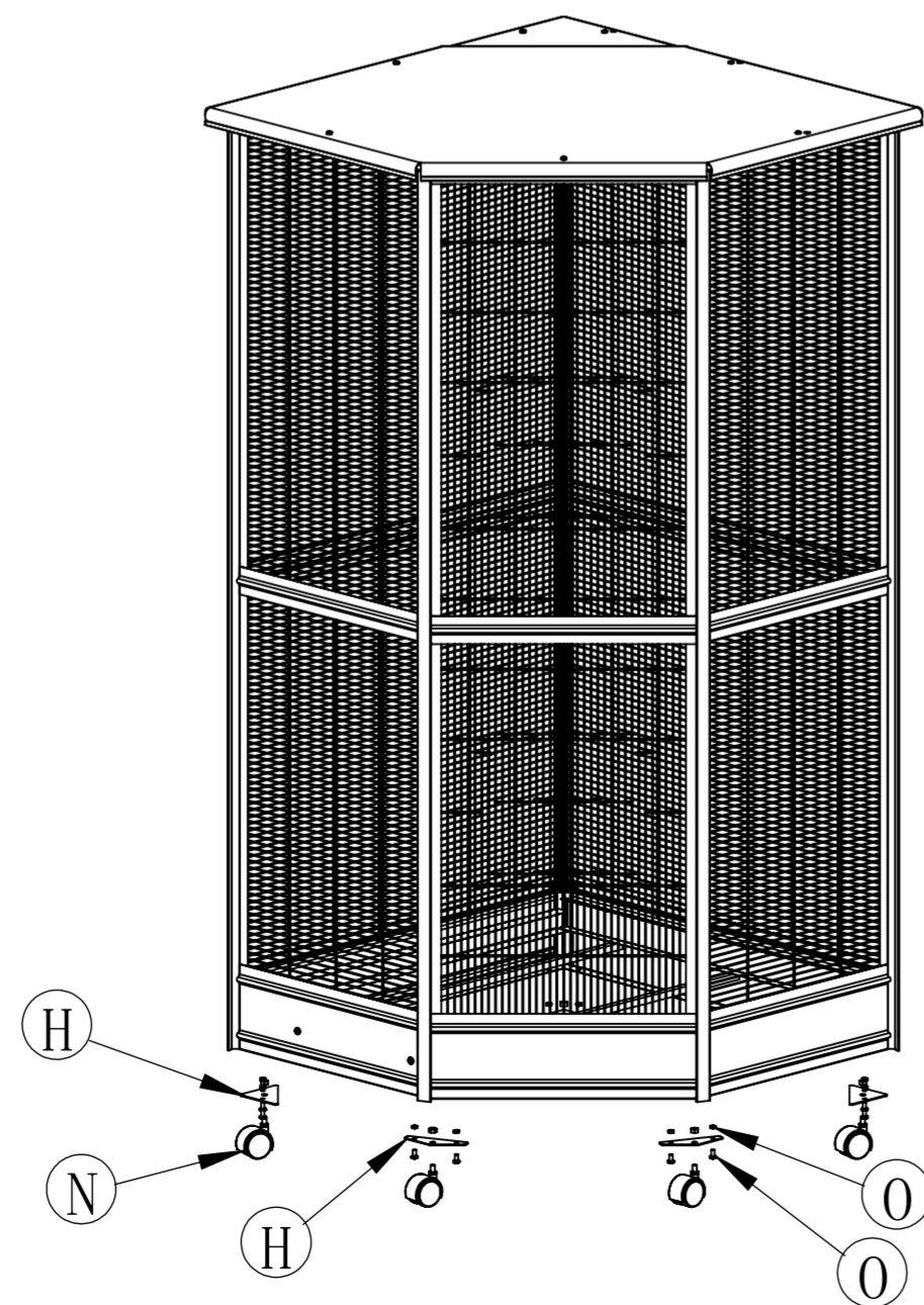
5、Screw the triangle plates H and wheels N to the cage bottom.
